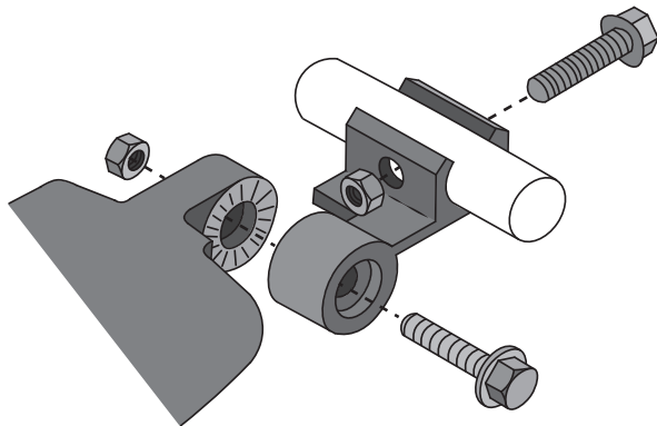
Bridge Mount
